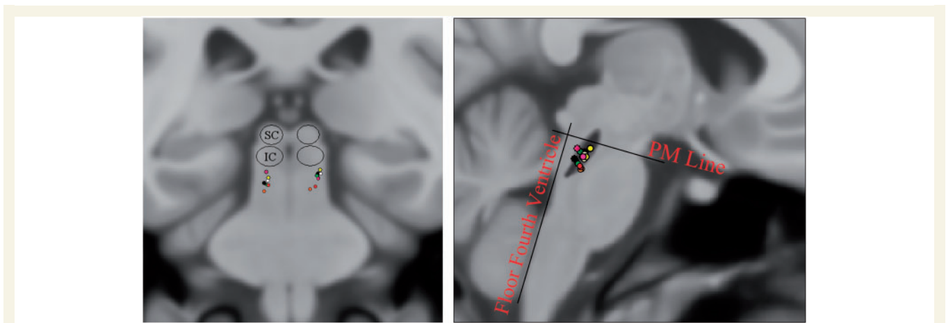
Figure 1 Localization of stimulation locations (coloured dots) represented in Montreal Neurological Institute (MNI) space (sagittal and coronal views). The relative location/extent of the pedunculopontine nucleus has been outlined on the sagittal view, based on choline-acetyltransferase immunohistochemical (ChAT5) staining in the human. Coordinates were calculated in millimetres from midline (laterality), ventrodorsal distance ( d ) from floor of the fourth ventricle and rostro-caudal distance ( h ) from a pontomesencephalic line connecting the pontomesencephalic junction to the inferior colliculi caudal margin, as described previously (Ferraye et al. , 2009). The mean (ranges) of these stimulation site coordinates were as follows: laterality 7.1 mm (4.6–9 mm), ventrodorsal distance ( d ) 5.8 mm (4.1–7.4 mm), rostro-caudal distance ( h ) -5.3 mm ( -2.2 to -8.0 mm). In Montreal Neurological Institute space, the coordinates relative to the anterior commissure for the average stimulation location, was as follows; X = 7.1 mm, Y = -32 mm, Z = -22 mm. PM = ponto-mesencephalic line connecting the pontomesencephalic junction to the caudal end of the inferior colliculi; SC = superior colliculus; IC = inferior colliculus.
